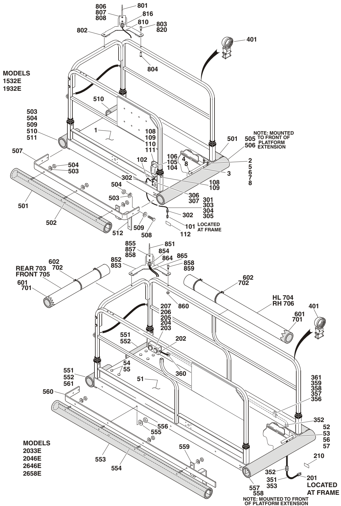
FIGURE 4-1. PLATFORM INSTALLATION - MANUALLY OPERATED EXTENSION
