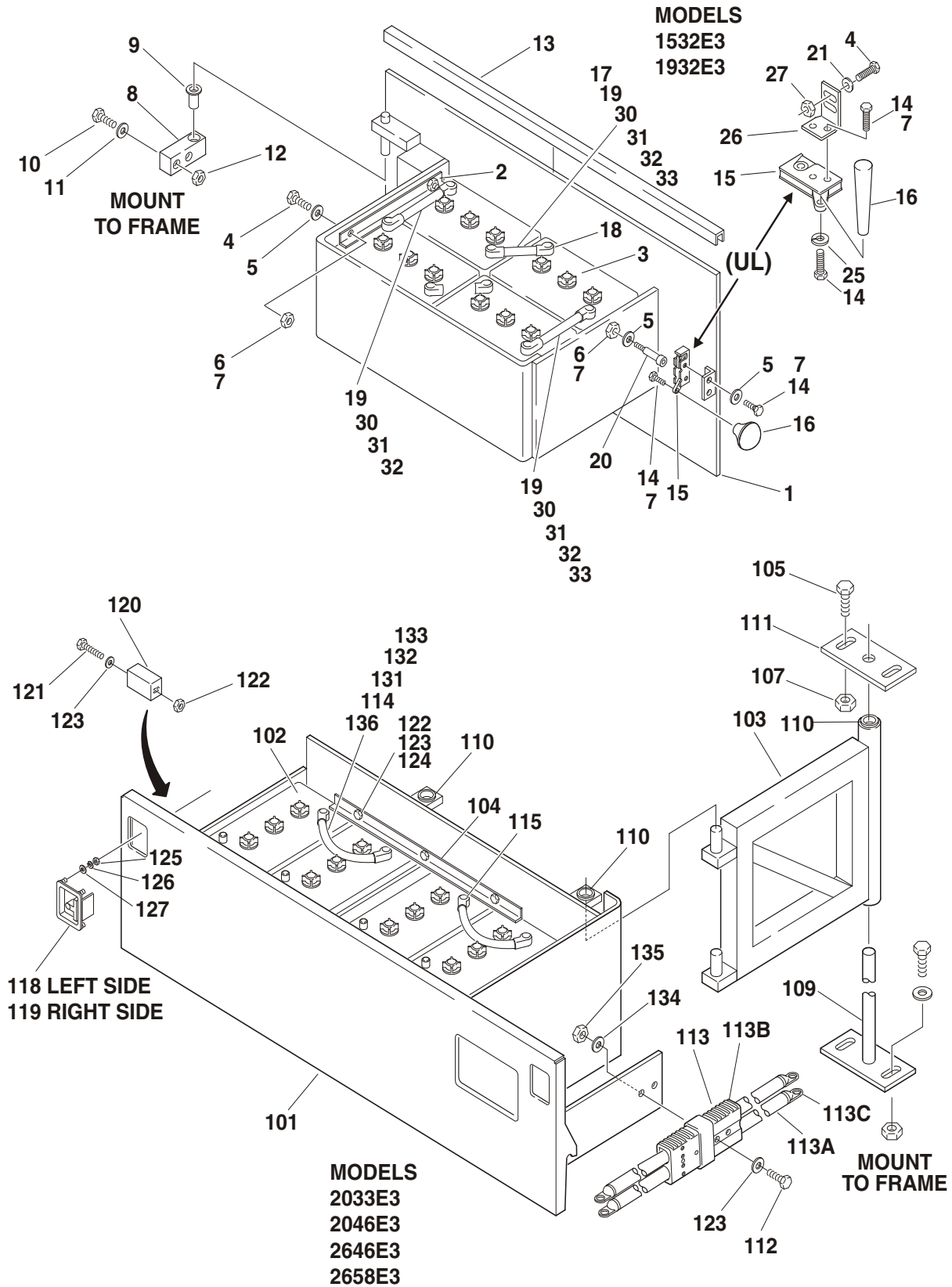
FIGURE 2-5. BATTERY INSTALLATIONS
