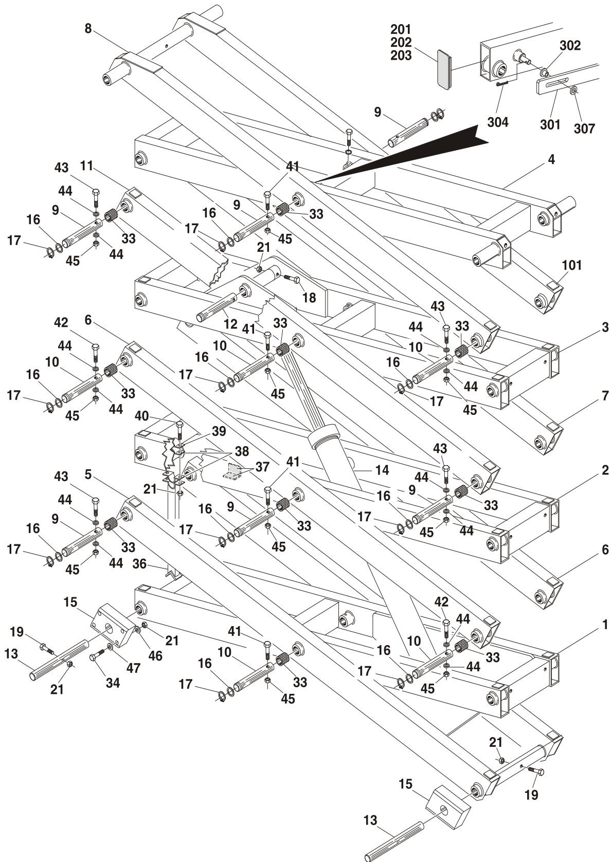
FIGURE 3-2. SCISSOR ARMS INSTALLATION - 1932E3
