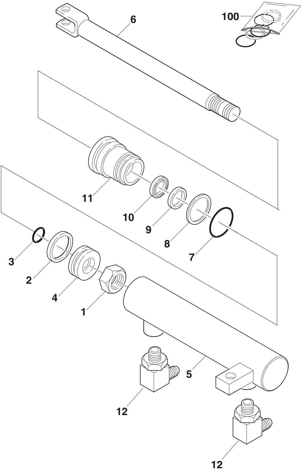
FIGURE 5-9.STEER CYLINDER ASSEMBLY (S/N 0200105071 TO PRESENT)
