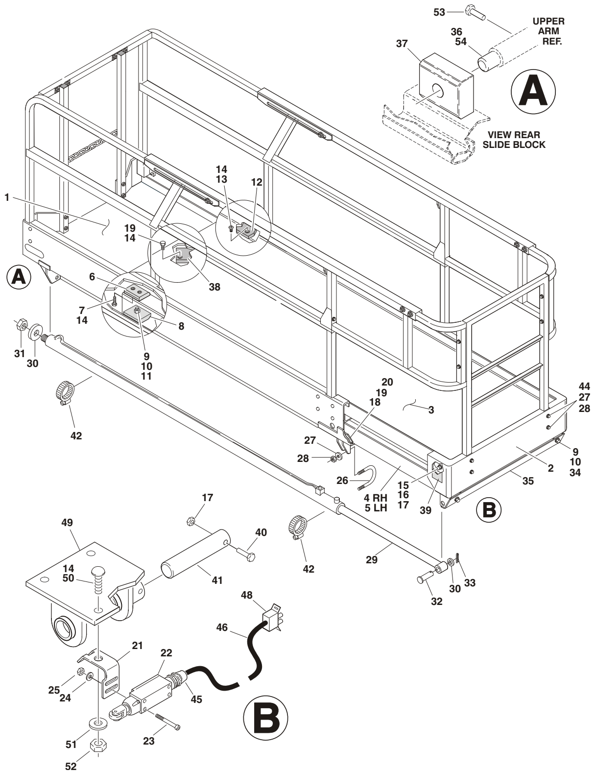
FIGURE 4-8. PLATFORM AND EXTENSION INSTALLATION - POWER OPERATED (2033E3/2046E3/2646E3/2658E3)
