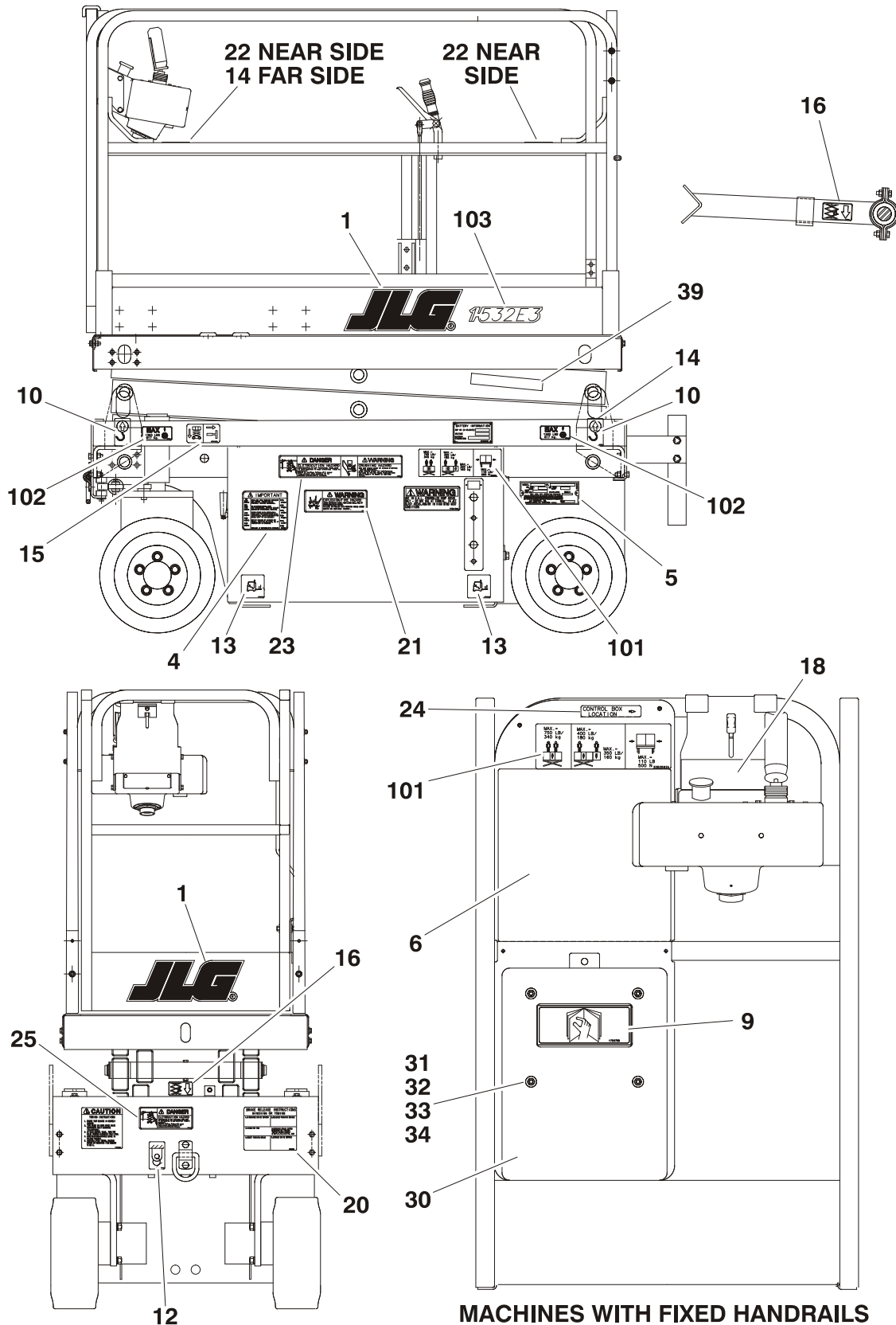
FIGURE 8-1.DECALS INSTALLATION - 1532E3/1932E3
