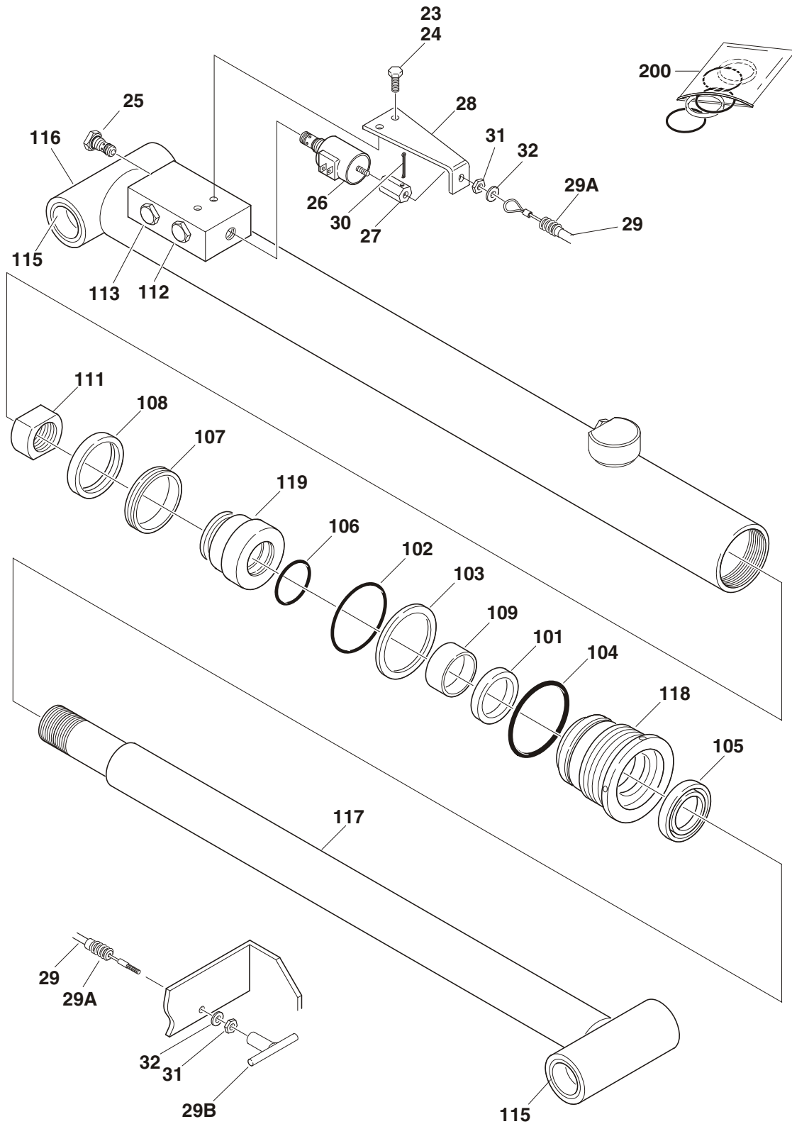
FIGURE 5-3.LIFT CYLINDER COMPONENTS ASSEMBLY 2033E3/2046E3
