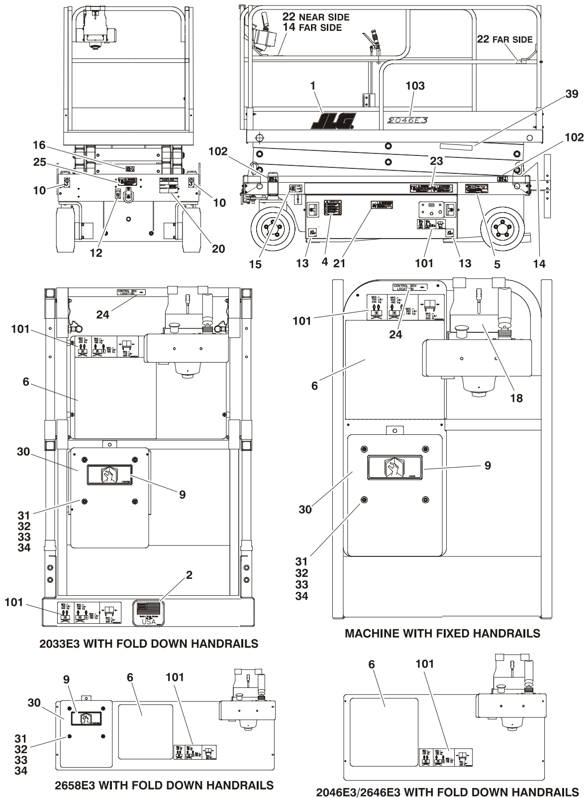
FIGURE 8-2.DECALS INSTALLATION - 2033E3/2046E3/2646E3/2658E3
