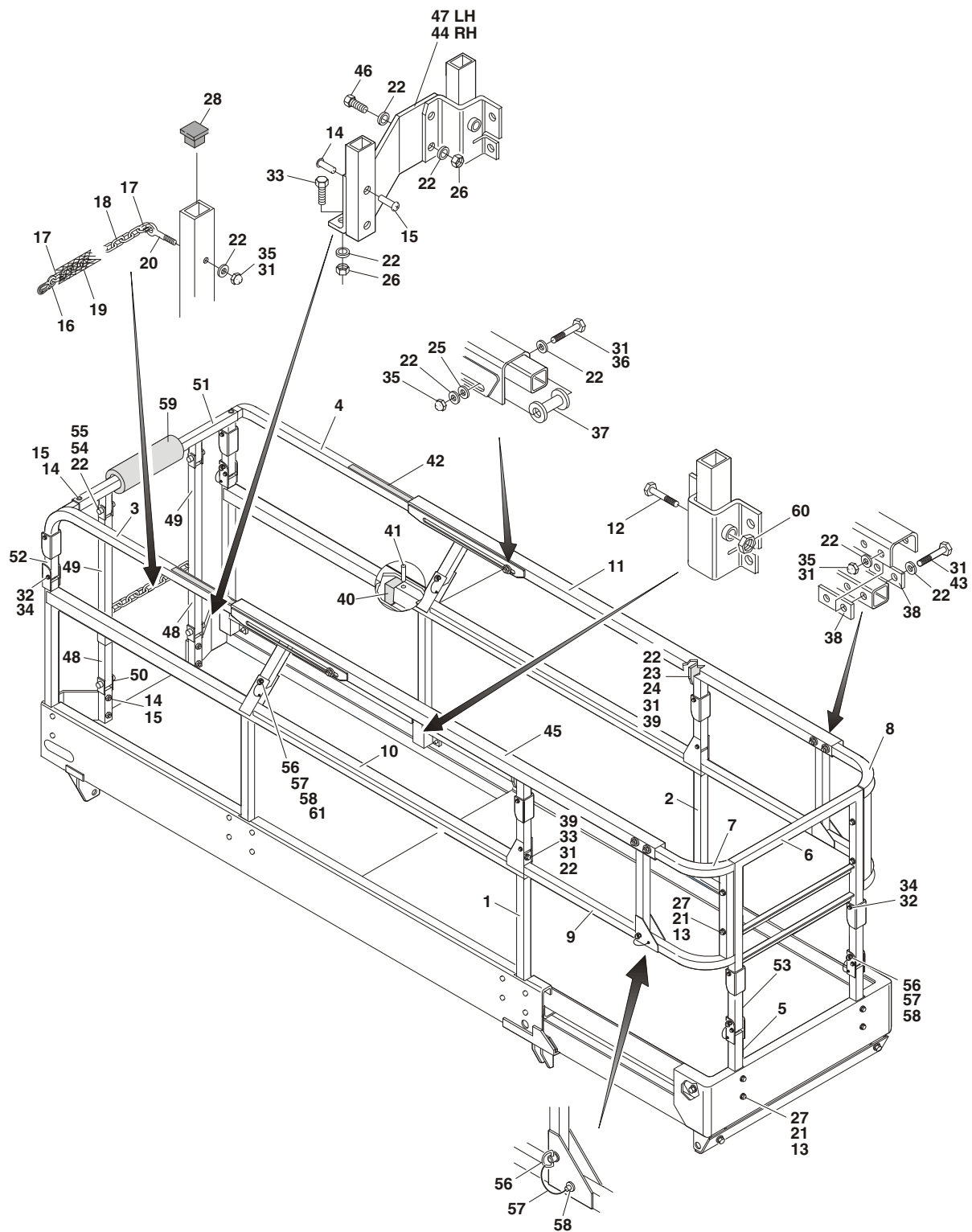
FIGURE 4-10. HANDRAILS INSTALLATION - FOLDDOWN HANDRAILS (POWER OPERATED EXTENSION) (2046E3/2646E3)
