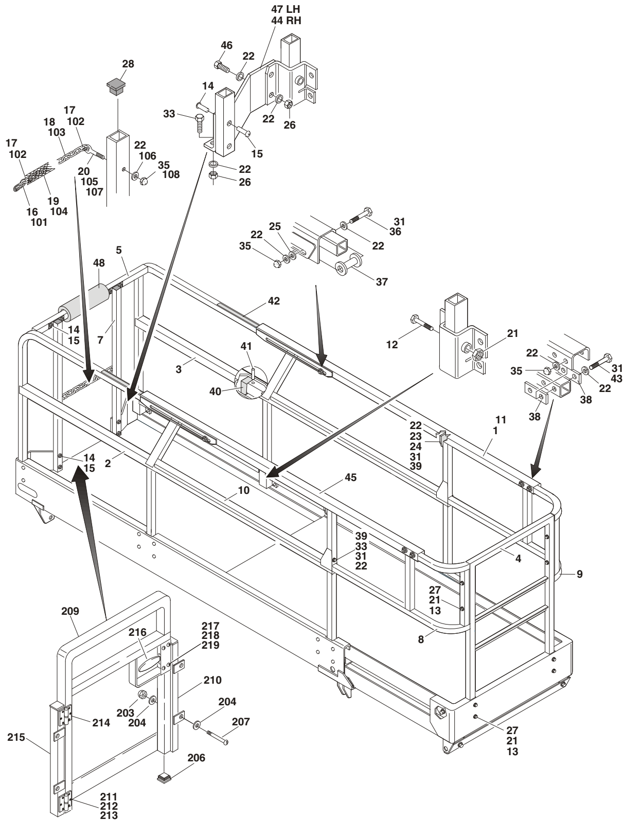
FIGURE 4-9. HANDRAILS INSTALLATION - STANDARD HANDRAILS (POWER OPERATED EXTENSION) (2033E3/2046E3/2646E3/2658E3)
