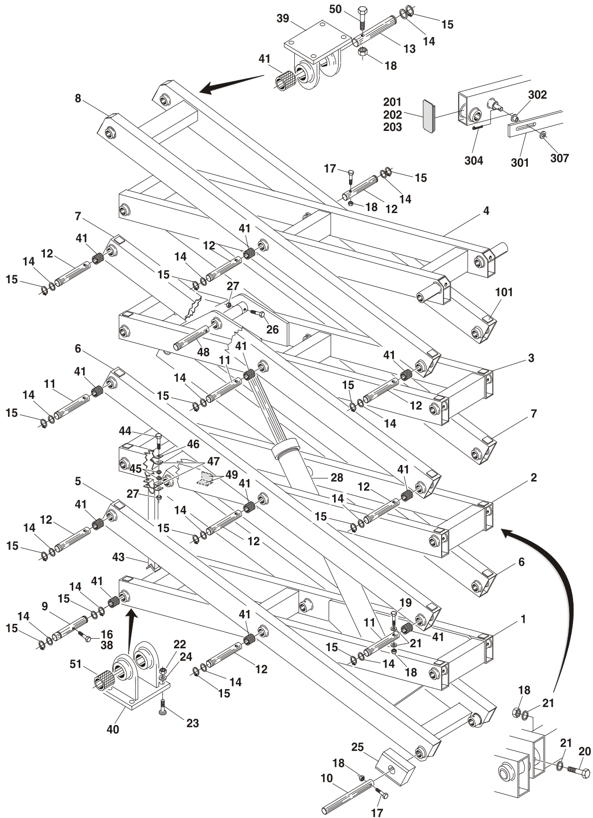
FIGURE 3-5. SCISSOR ARMS INSTALLATION - 2646E3/2658E3
