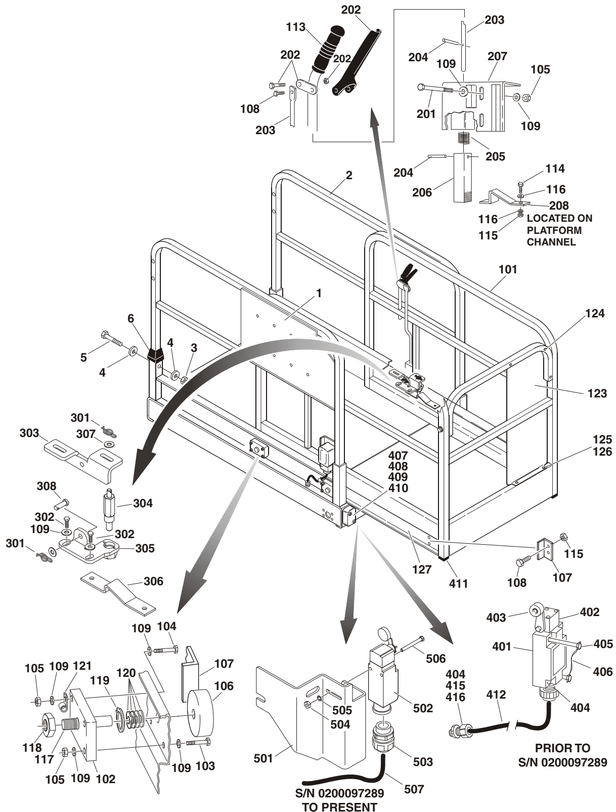
FIGURE 4-2. HANDRAILS AND EXTENSION INSTALLATION - STANDARD HANDRAILS (MANUALLY OPERATED EXTENSION) (1532E3/1932E3)
