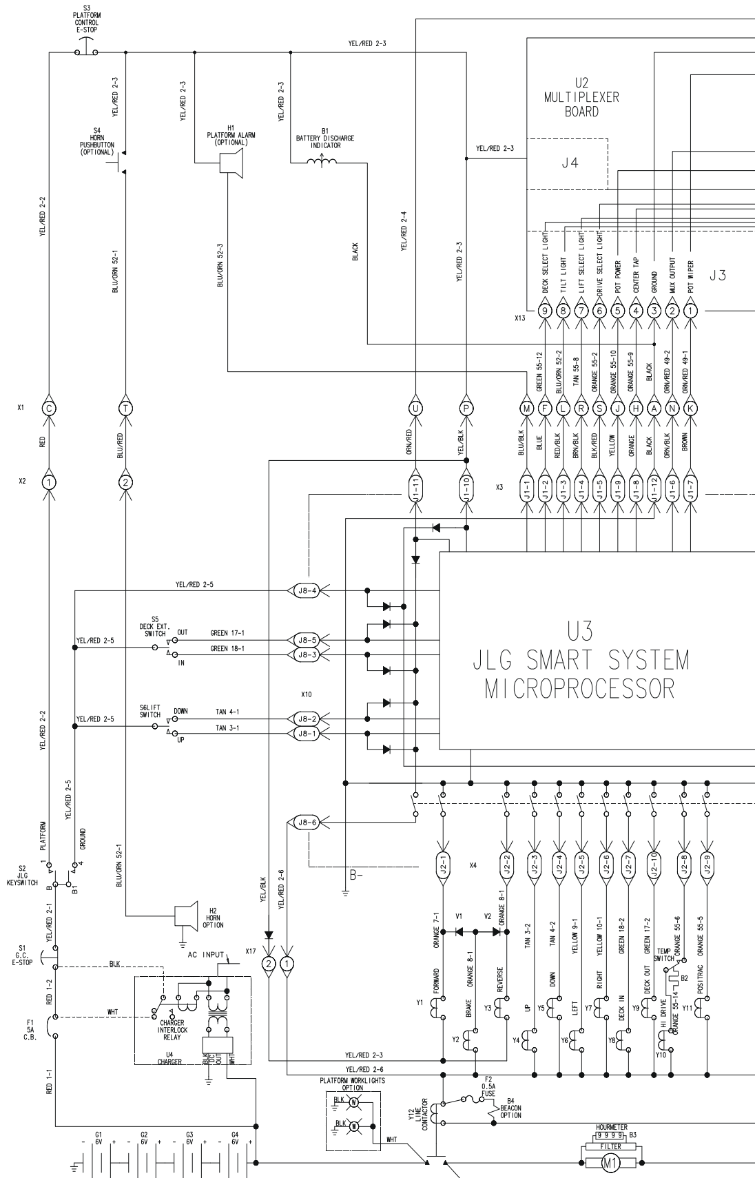
FIGURE 7-2.ELECTRICAL SCHEMATIC - STANDARD
