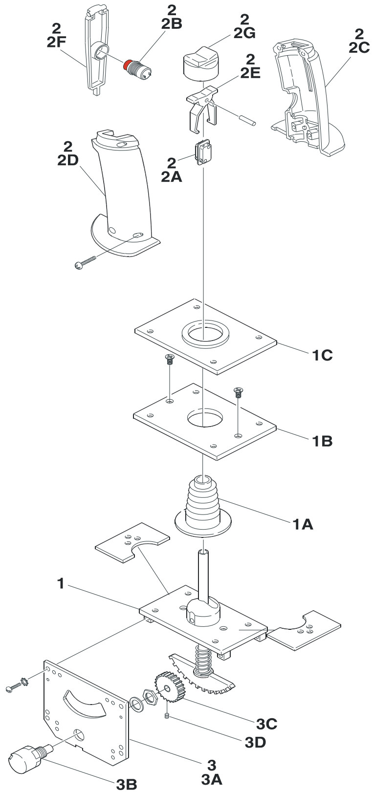
FIGURE 4-12.CONTROLLER ASSEMBLY - PQ
