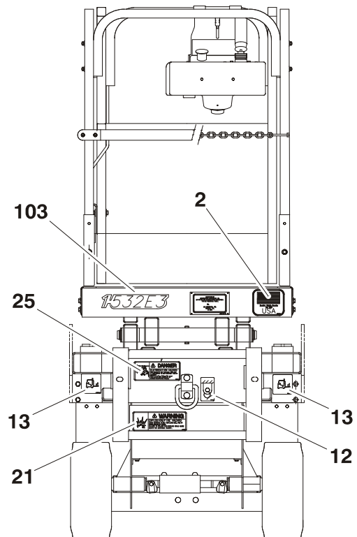
MACHINES WITH FOLDDOWN HANDRAILS
