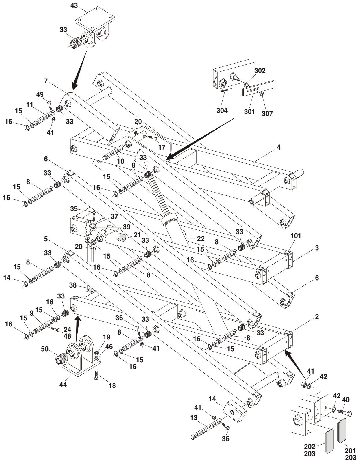
FIGURE 3-3. SCISSOR ARMS INSTALLATION - 2033E3
